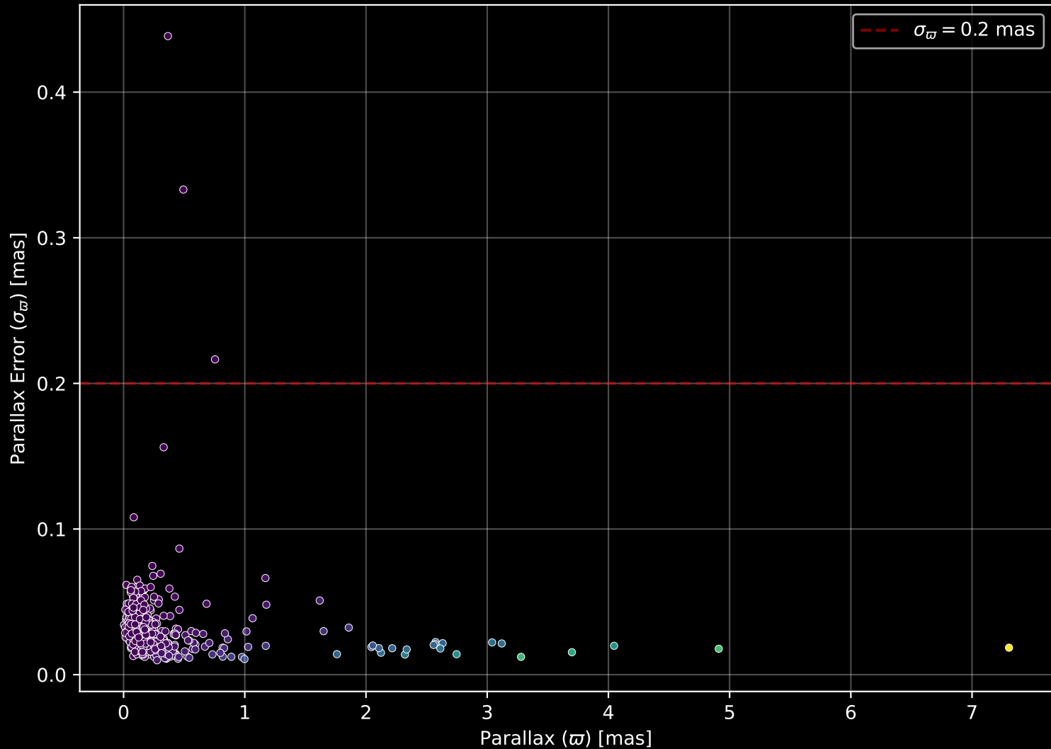
APOGEE DR17 Field: [100+06] Parallax Quality (n= 556)
