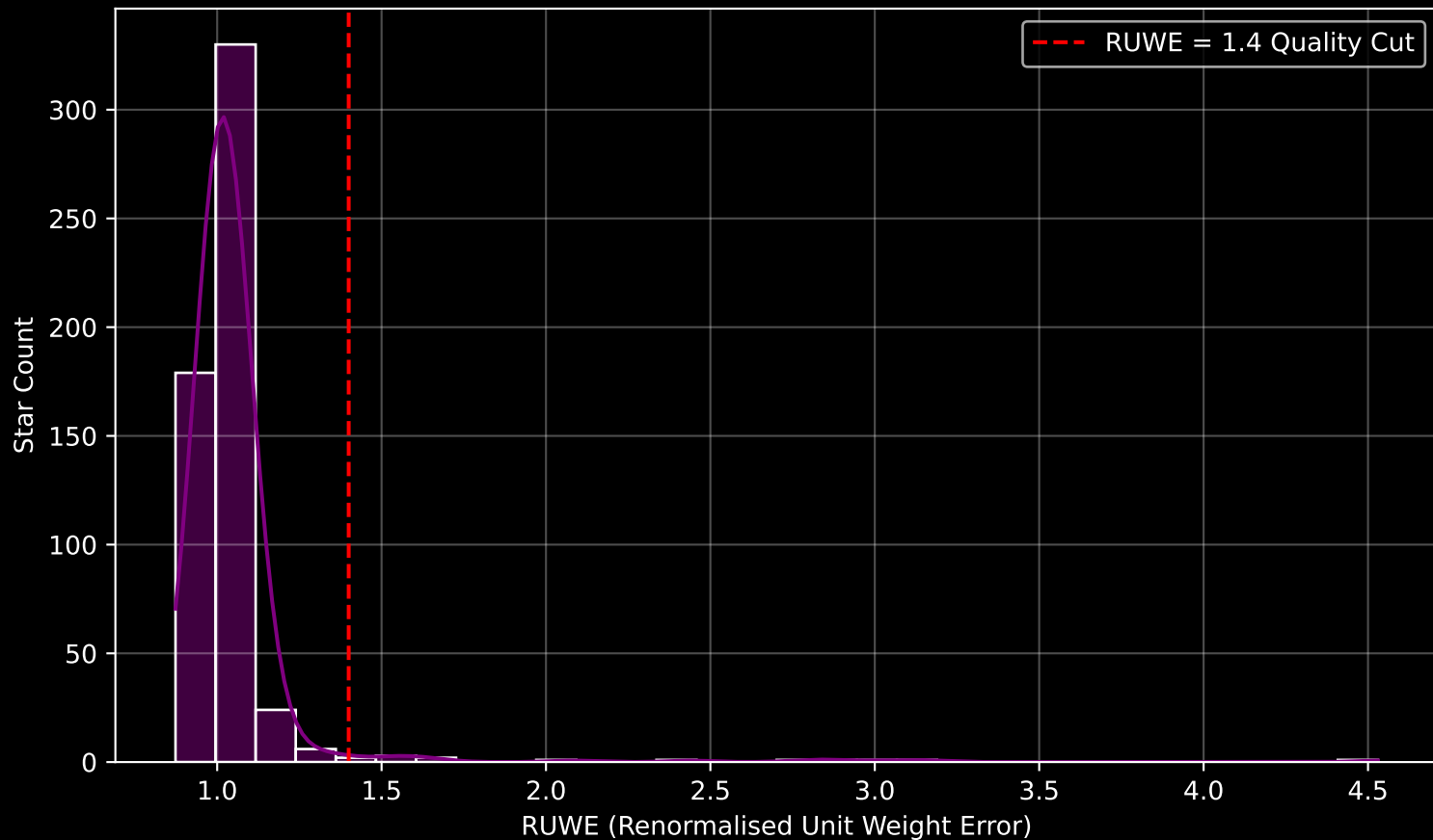
GAPOGEE DR17 Field [100+06] RUWE Distribution (n= 553)
