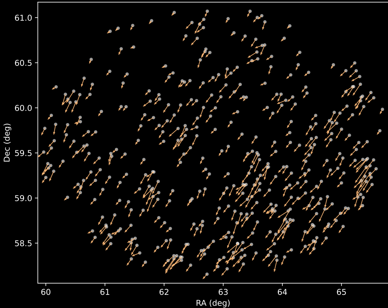
APOGEE DR17 Cluster 3 Proper Motion Vectors (n=424)
