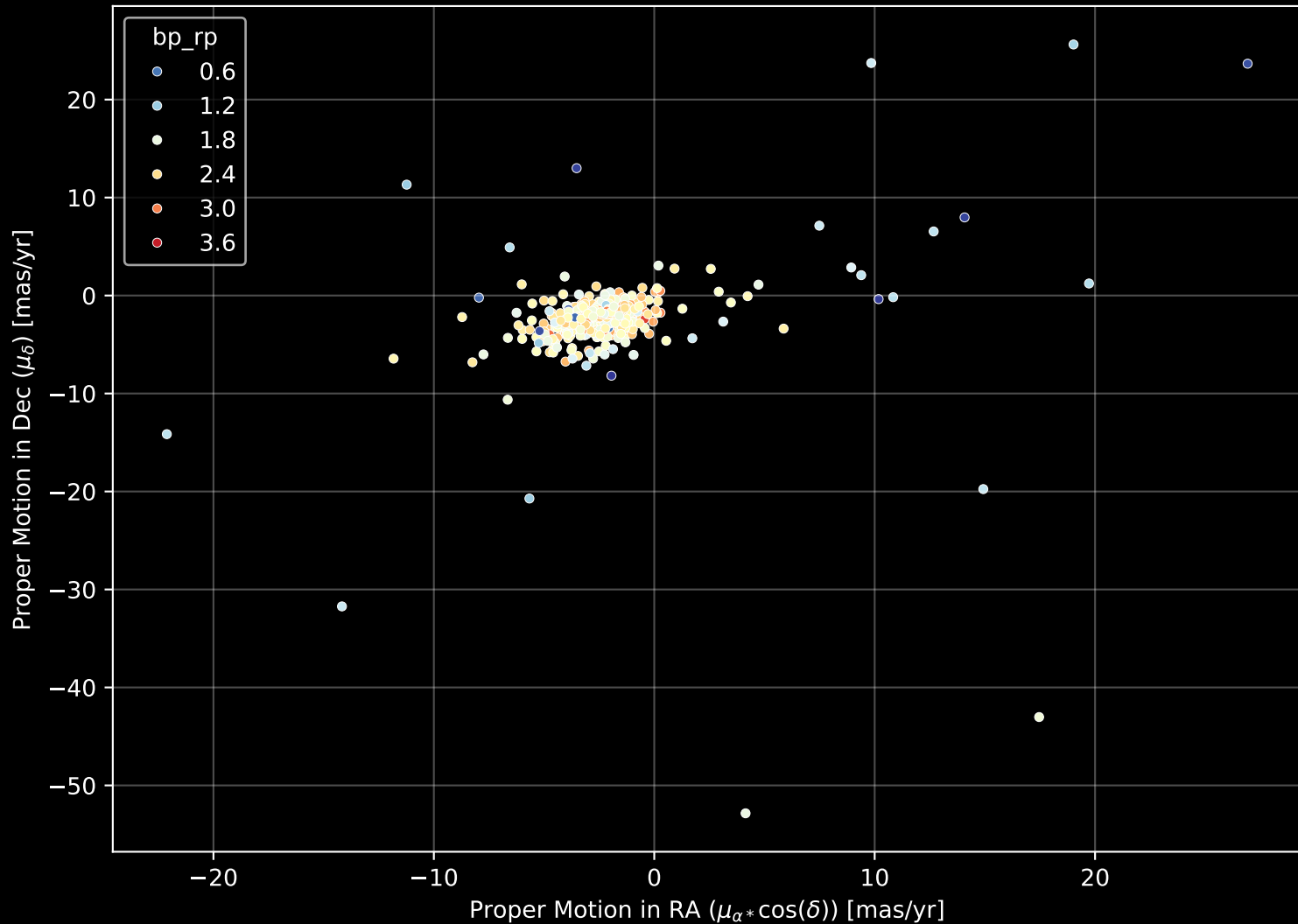
APOGEE DR17 Field: [100+06] Proper Motion Diagram (n= 556)
