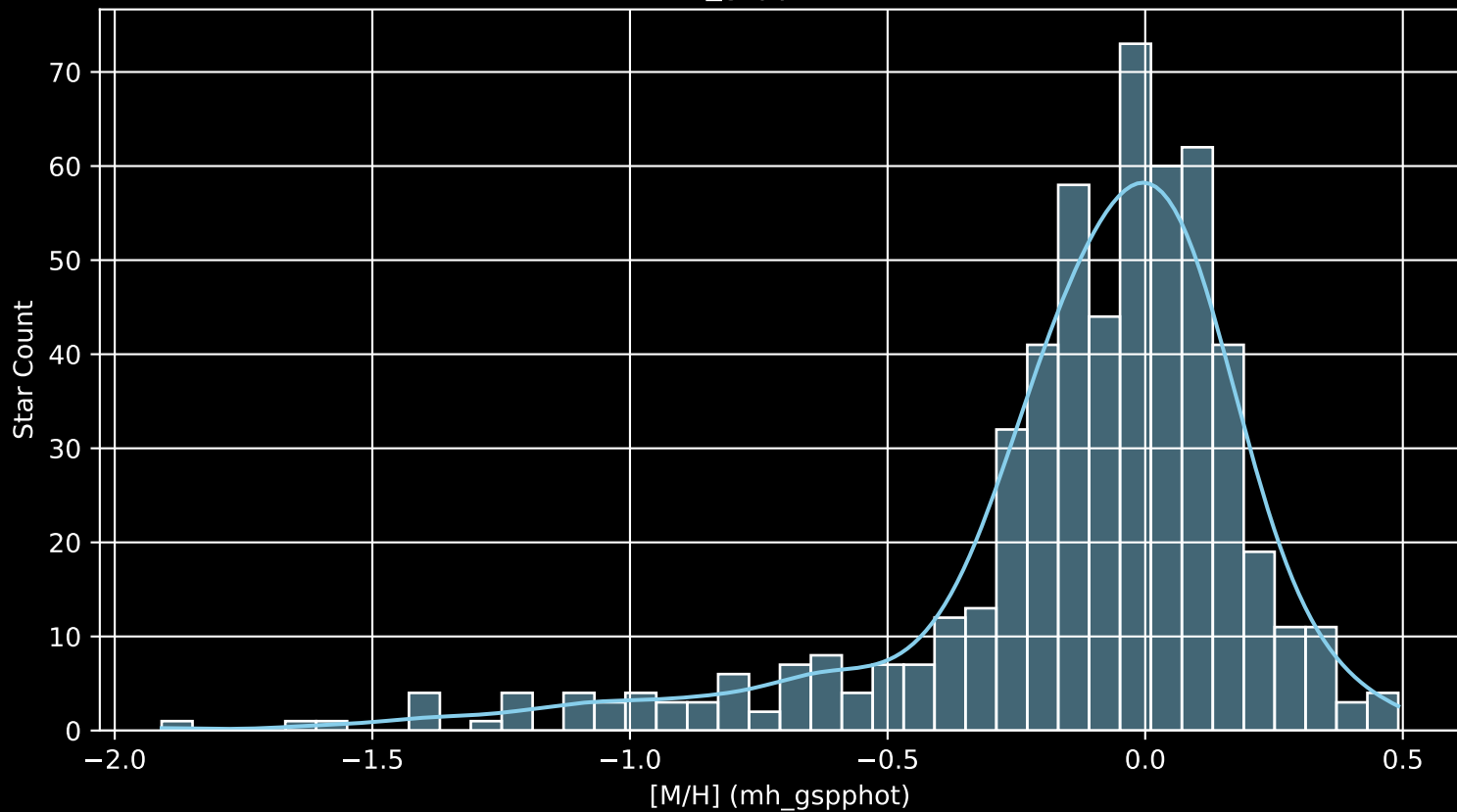
APOGEE DR17 Field: [100+06 [M/H] (mh_gspphot) (n= 554)
