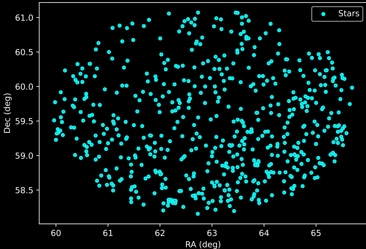
APOGEE DR17 Field: [100+06] Proper Motion Vectors for Gaia Star Field (n= 556)
